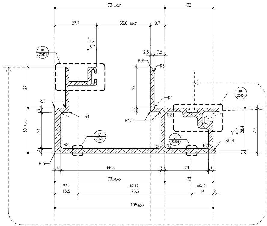
B1 TYPICAL MALE MULLION SCALE 1:1 @ A3
