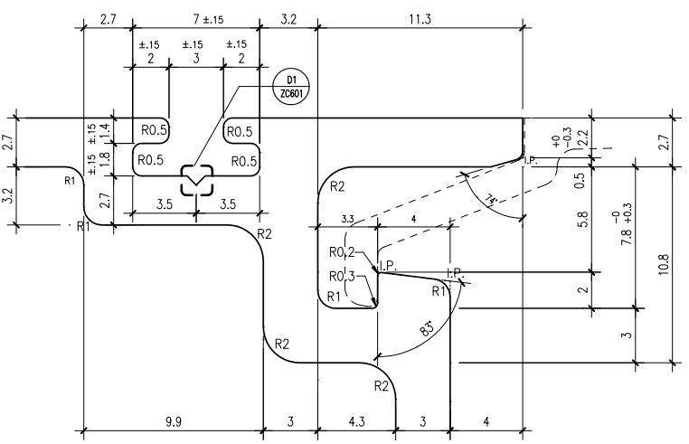
D4 BLOW UP DETAIL – TYPICAL MALE MULLION NOT TO SCALE
