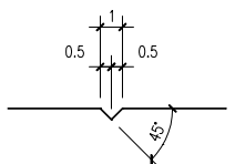
D1 BLOW UP DETAIL – TYPICAL MALE MULLION NOT TO SCALE
