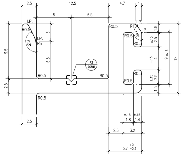
B4 BLOW UP DETAIL – TYPICAL MALE MULLION NOT TO SCALE
